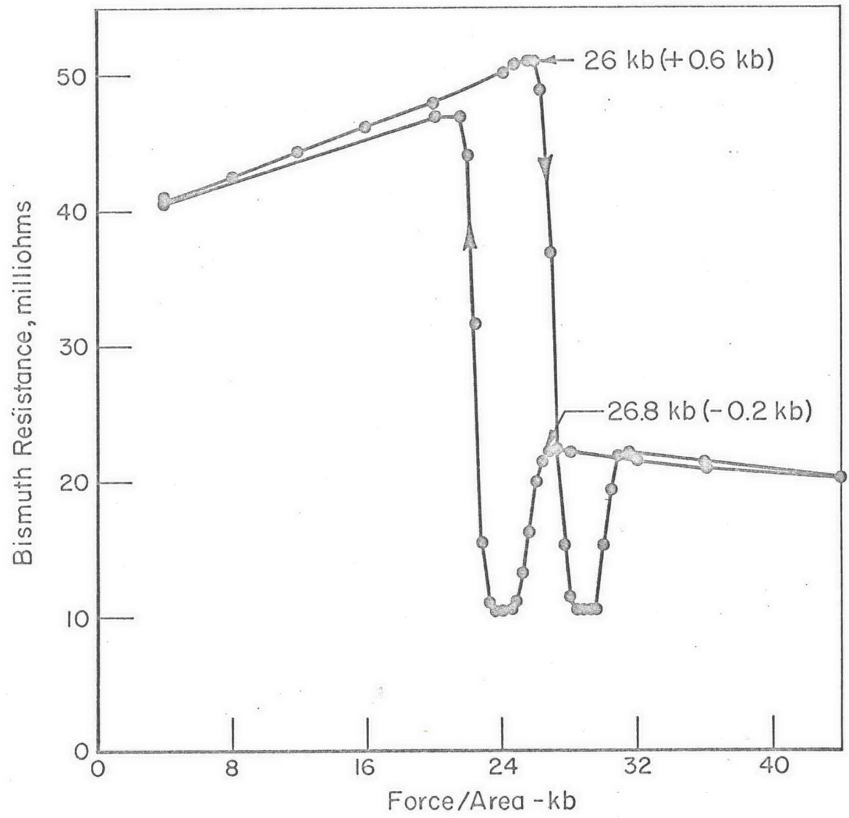
BISMUTH CALIBRATION IN AgCl PORTION OF CELL
